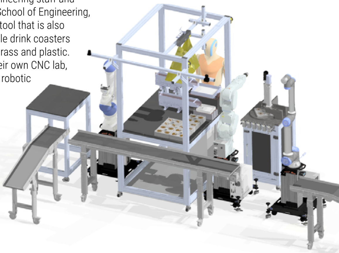
Flexible Production Assembly Cell (Flex-PAC)
